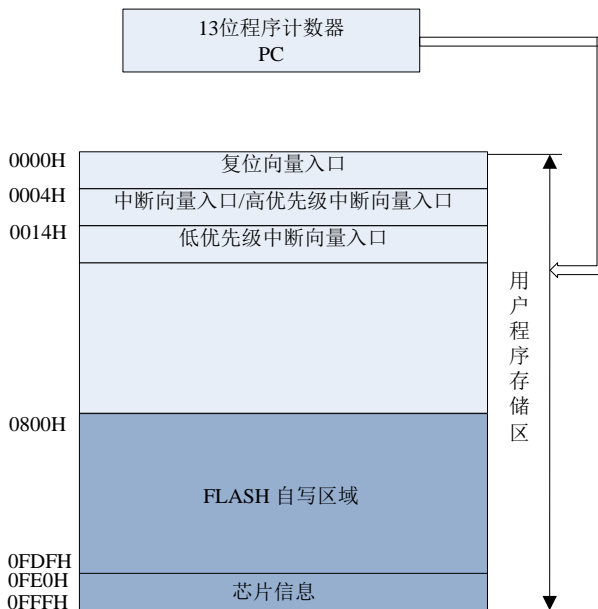
图 3.3 KF8F3110/12/20/22/30/32 程序存储器映射
